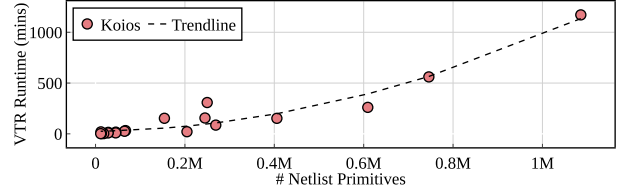
Fig. 1: VTR runtime for the Koios benchmarks.
