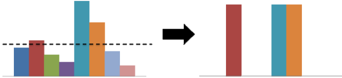
Fig. 6 Histogram binarization
