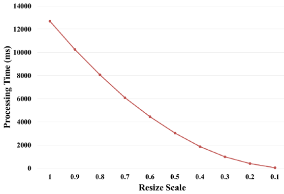
Fig. 12 Resize down scale vs. processing time
